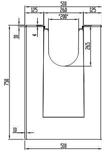
Trash box with galvanised mud bucket view from the front 2
