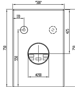
Trash box with galvanised mud bucket view from the side
