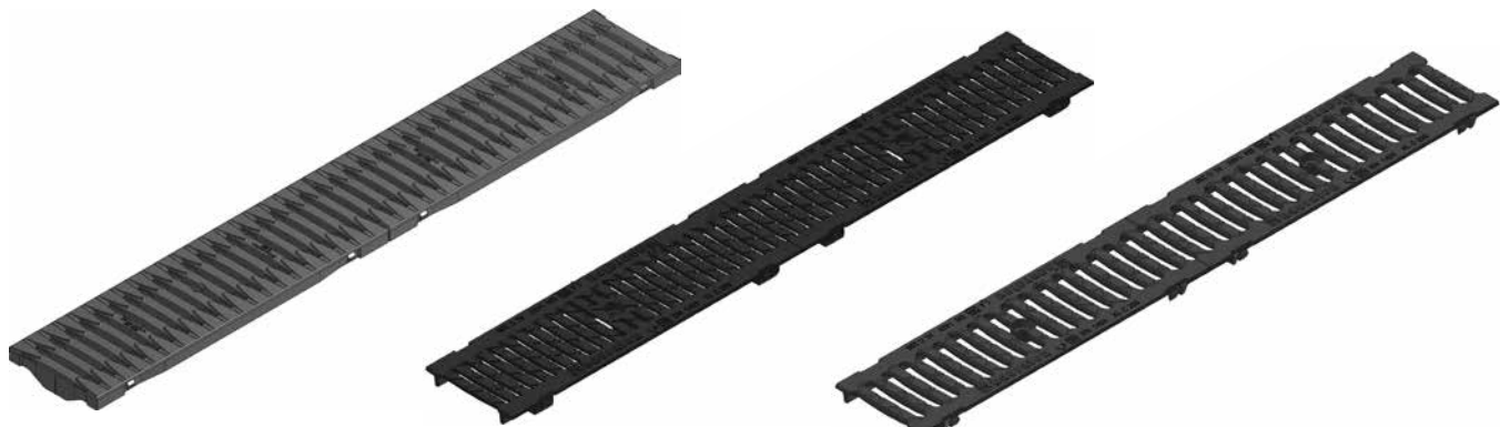
FIBRETEC design slotted grating in the colour Black, SW 9 mm
