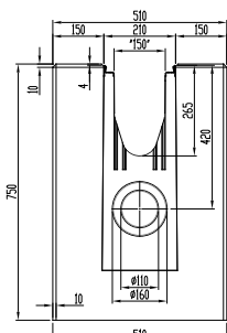
Trash box with galvanised mud bucket view from the front 1
