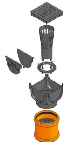
TOP X universal box, black, with connection set, end caps, leaf trap, foul air trap, inclusive assembly instruction
